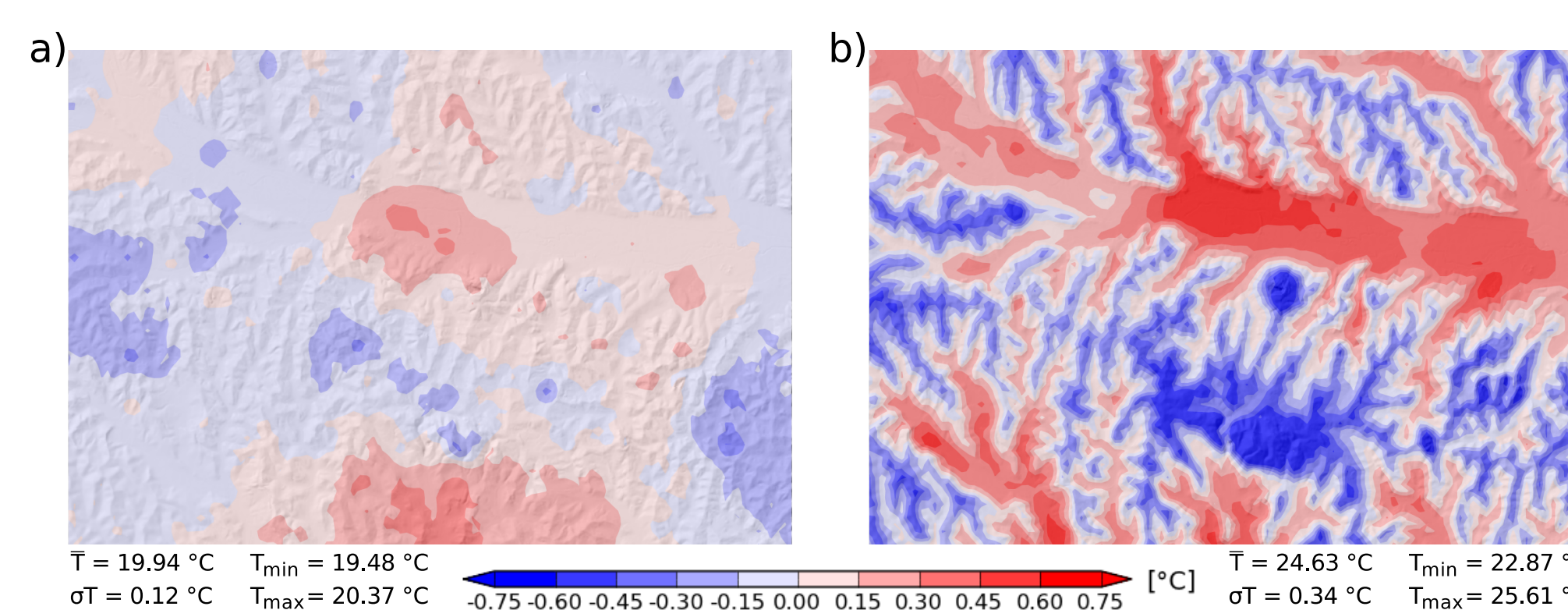
Fig. 3: Spatial grids of WegenerNet FBR climatological temperature data for July 2008. (a) Monthly-mean temperature anomaly and (b) monthly-mean temperature anomaly after noontime (13:00-14:00 LT).
