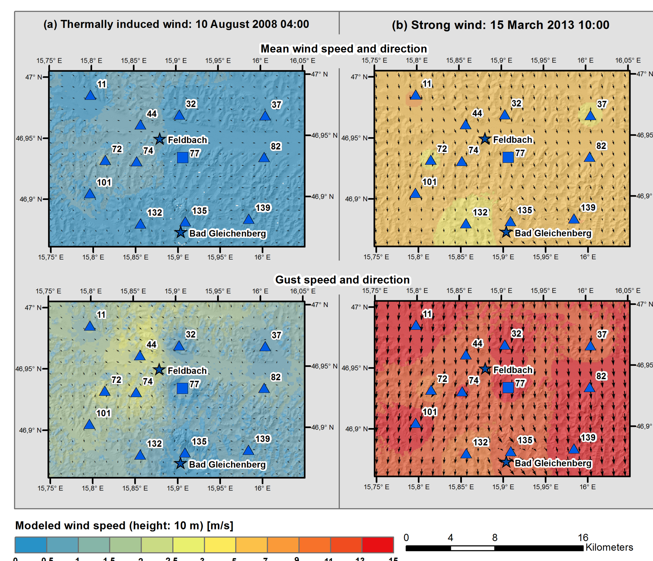
Fig. 5: High-resolution windfields derived from data of the 12 WegenerNet FBR wind stations (blue symbols). (a) Thermally induced (weak) wind on Aug. 10, 2008. Upper image: mean, lower image: gusts. (b) Strong northerly wind on March 15, 2013. Upper image: mean, lower image: gusts.
